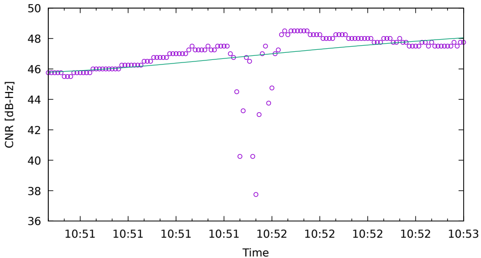
CNR fit for C28 on SamsungS20 - drive 7 (DOY263)
