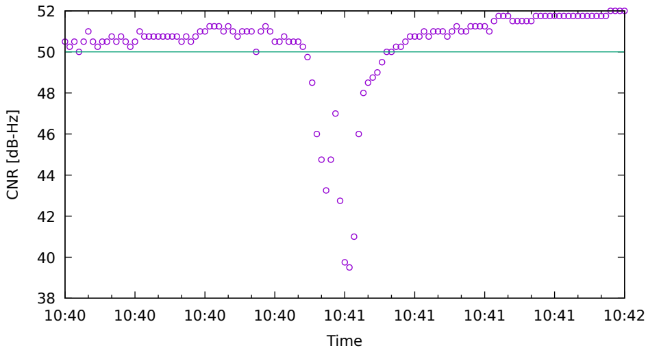
CNR fit for C33 on SamsungS20 - drive 1 (DOY263)
