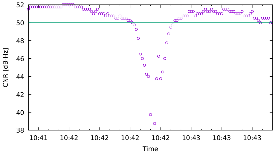
CNR fit for C33 on SamsungS20 - drive 2 (DOY263)
