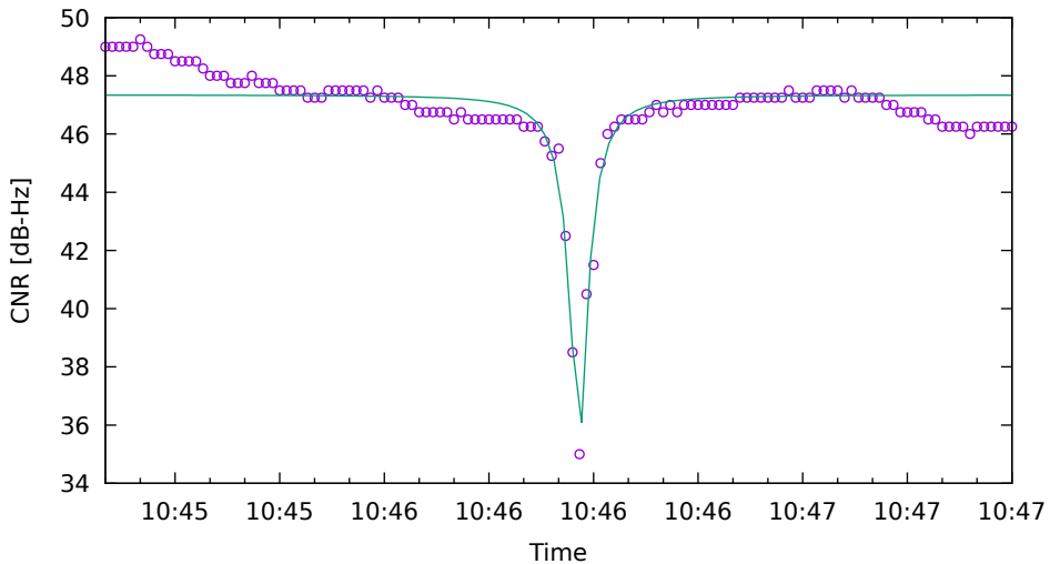
CNR fit for C33 on SamsungS20 - drive 4 (DOY263)
