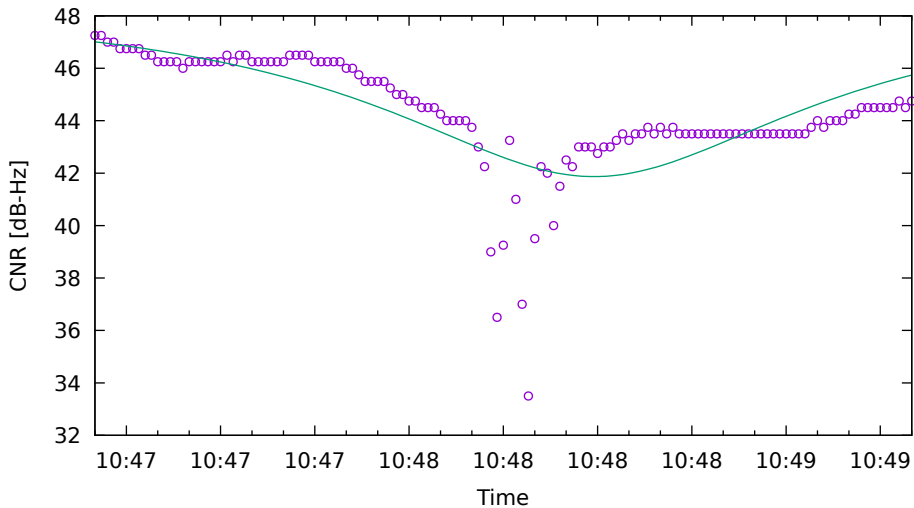
CNR fit for C33 on SamsungS20 - drive 5 (DOY263)
