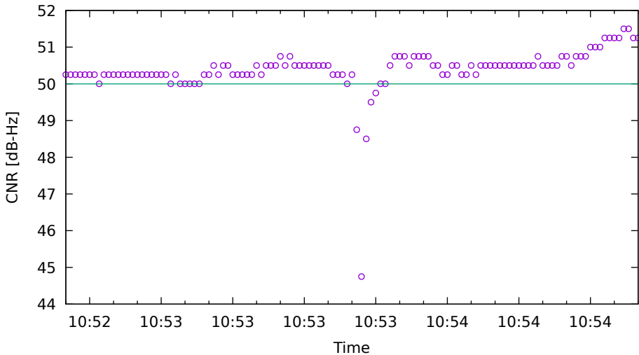
CNR fit for C33 on SamsungS20 - drive 8 (DOY263)
