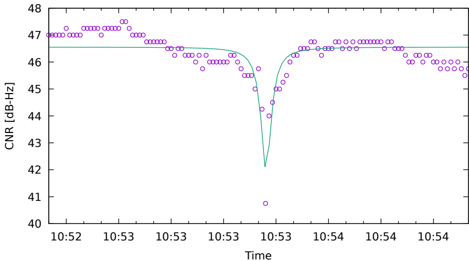
CNR fit for E04 on SamsungS20 - drive 8 (DOY263)
