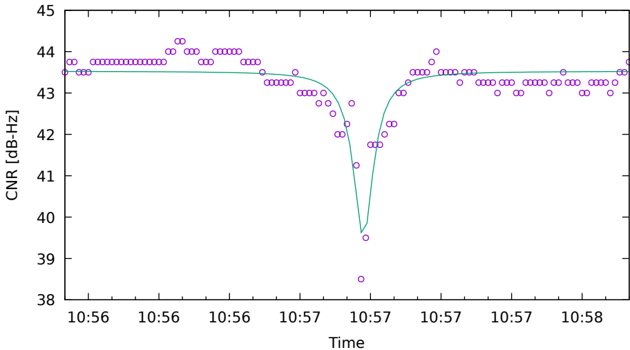
CNR fit for E11 on SamsungS20 - drive 10 (DOY263)
