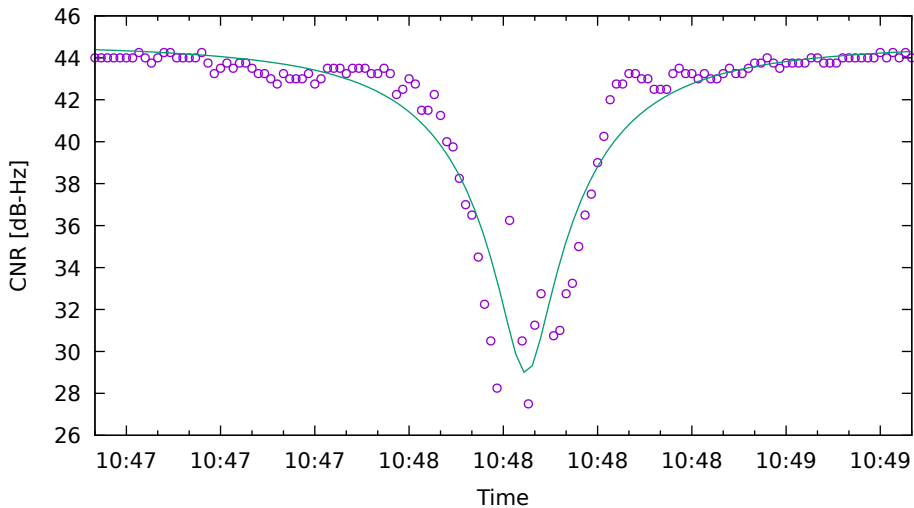
CNR fit for E11 on SamsungS20 - drive 5 (DOY263)
