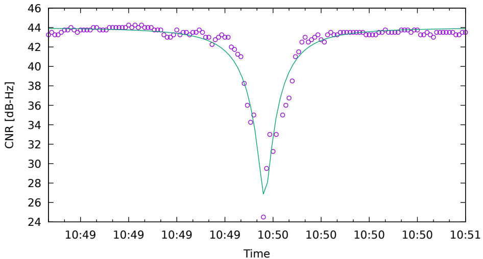
CNR fit for E11 on SamsungS20 - drive 6 (DOY263)
