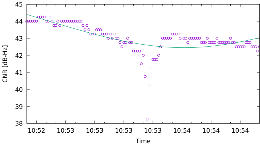
CNR fit for E11 on SamsungS20 - drive 8 (DOY263)
