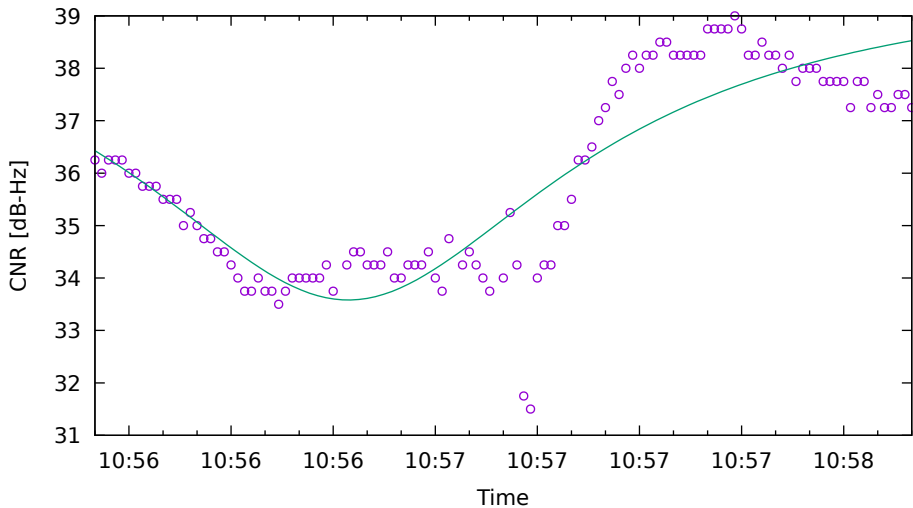
CNR fit for E19 on SamsungS20 - drive 10 (DOY263)
