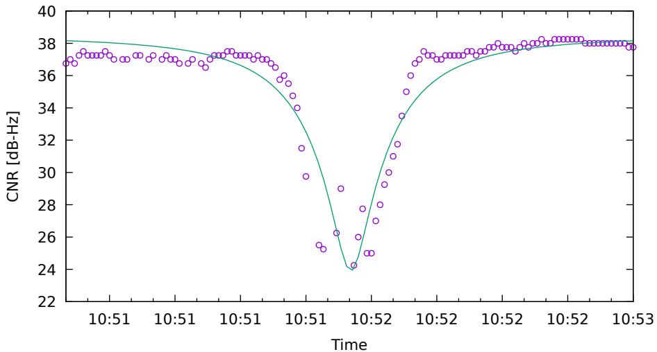
CNR fit for E19 on SamsungS20 - drive 7 (DOY263)
