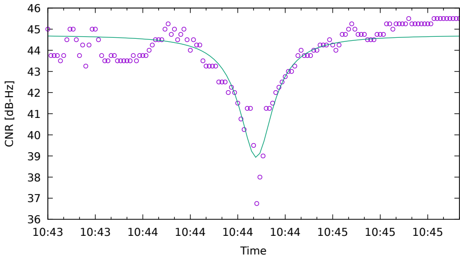
CNR fit for G04 on SamsungS20 - drive 3 (DOY263)
