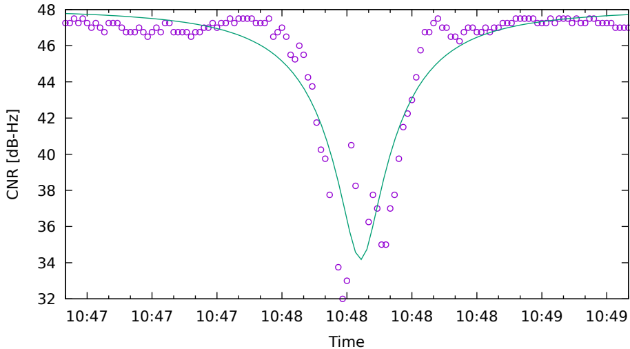
CNR fit for G06 on SamsungS20 - drive 5 (DOY263)
