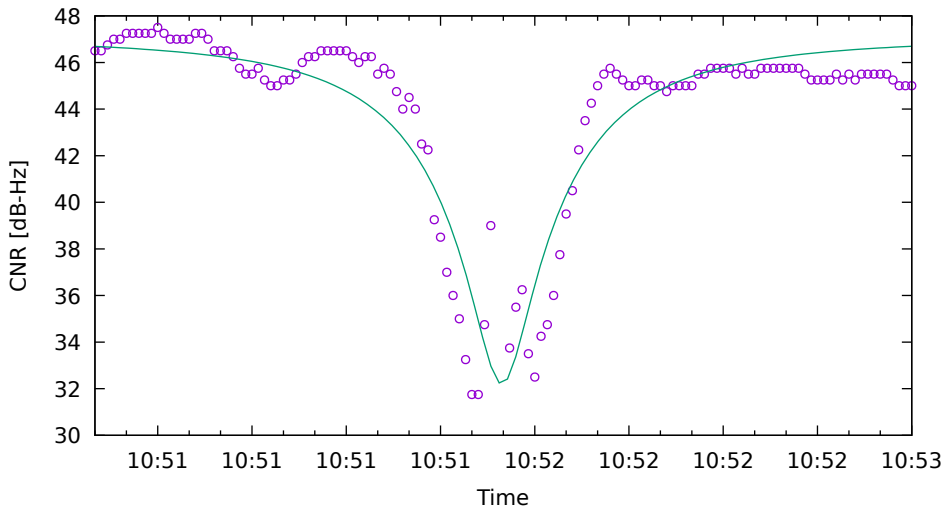
CNR fit for G06 on SamsungS20 - drive 7 (DOY263)
