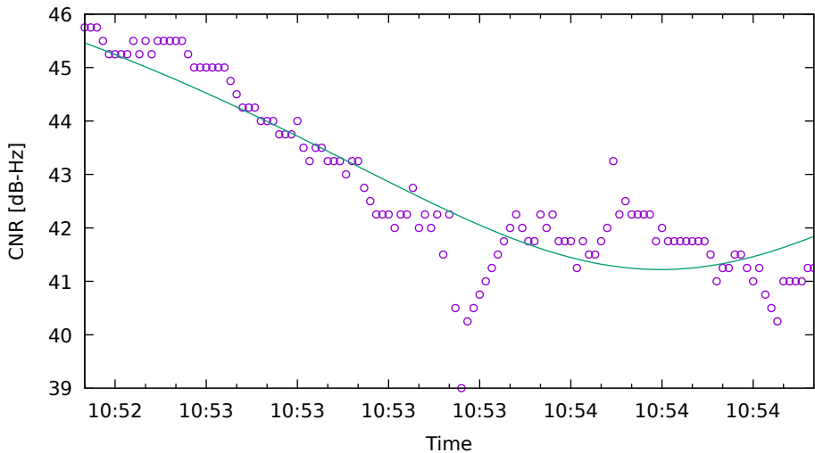
CNR fit for G06 on SamsungS20 - drive 8 (DOY263)
