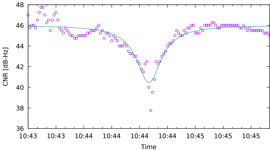
CNR fit for G09 on SamsungS20 - drive 3 (DOY263)
