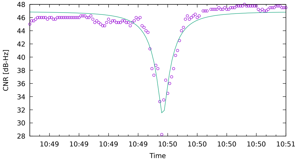
CNR fit for G09 on SamsungS20 - drive 6 (DOY263)
