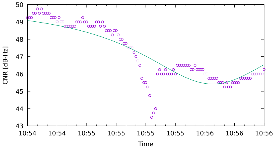
CNR fit for G09 on SamsungS20 - drive 9 (DOY263)
