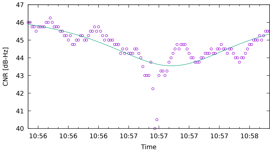
CNR fit for G21 on SamsungS20 - drive 10 (DOY263)
