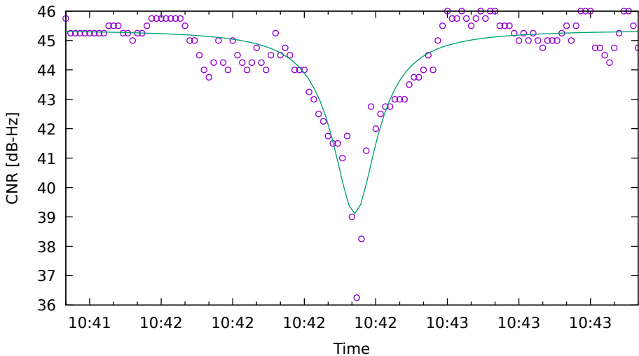
CNR fit for G21 on SamsungS20 - drive 2 (DOY263)
