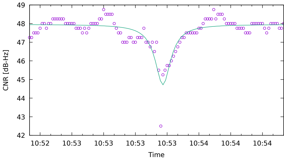
CNR fit for G21 on SamsungS20 - drive 8 (DOY263)
