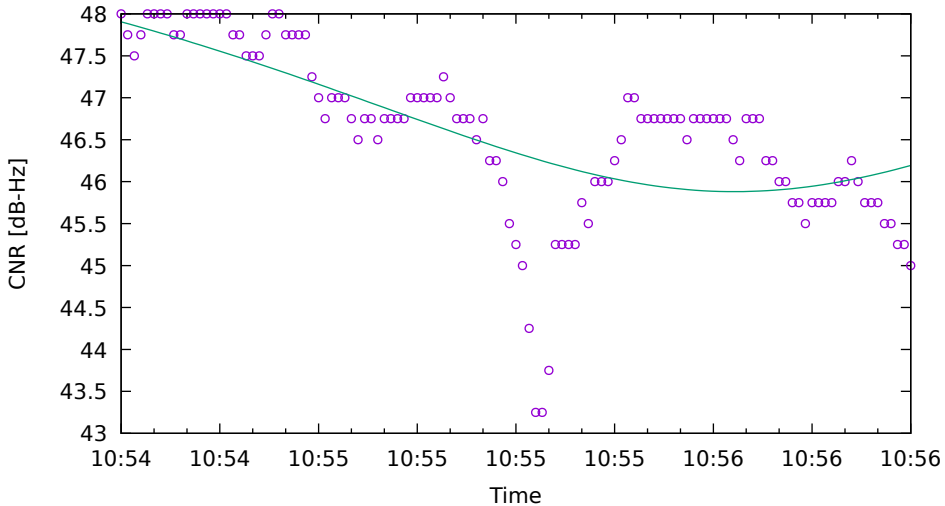
CNR fit for G21 on SamsungS20 - drive 9 (DOY263)
