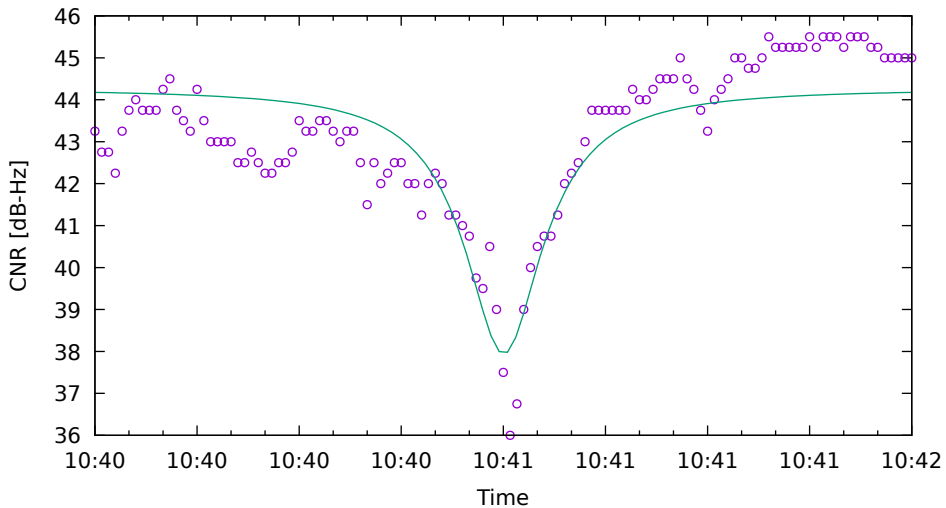
CNR fit for G31 on SamsungS20 - drive 1 (DOY263)
