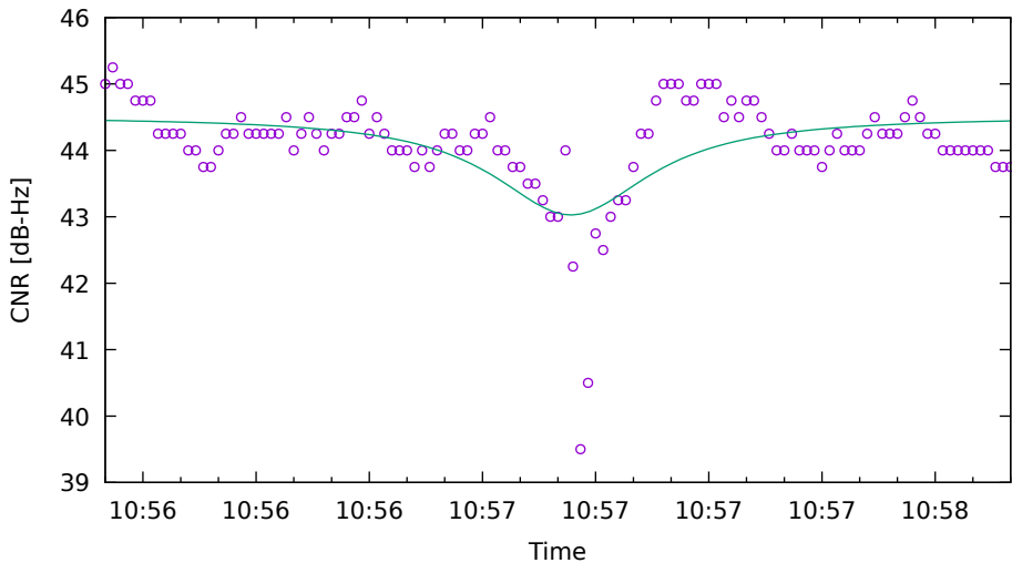
CNR fit for G31 on SamsungS20 - drive 10 (DOY263)
