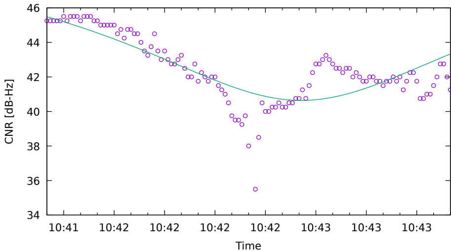
CNR fit for G31 on SamsungS20 - drive 2 (DOY263)
