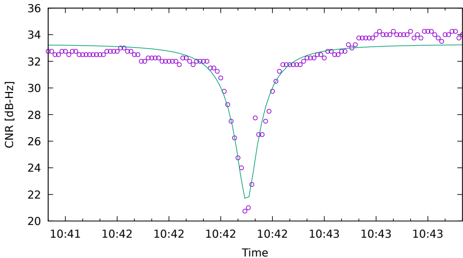
CNR fit for C09 on Xiaomi11T - drive 2 (DOY263)
