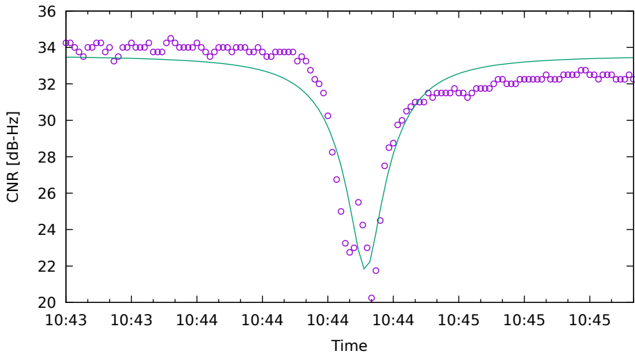
CNR fit for C09 on Xiaomi11T - drive 3 (DOY263)
