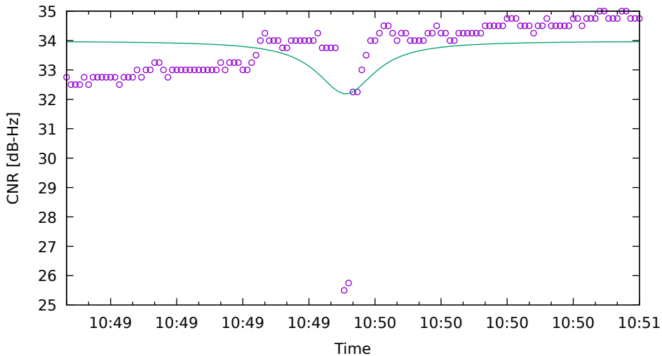
CNR fit for C09 on Xiaomi11T - drive 6 (DOY263)
