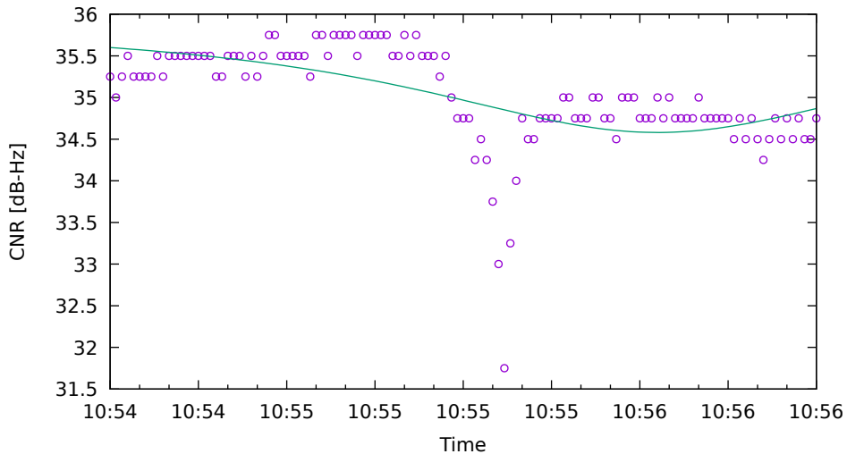
CNR fit for C09 on Xiaomi11T - drive 9 (DOY263)
