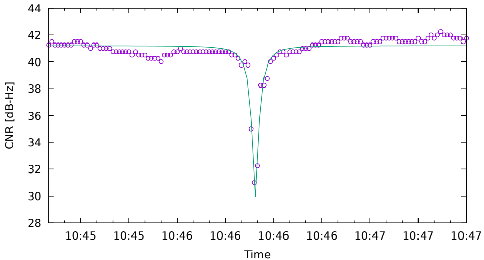
CNR fit for C11 on Xiaomi11T - drive 4 (DOY263)
