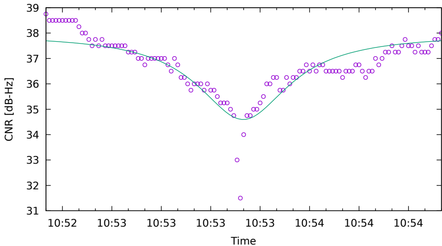
CNR fit for C11 on Xiaomi11T - drive 8 (DOY263)
