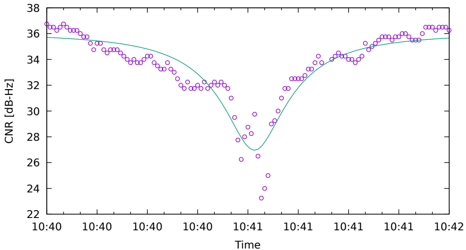
CNR fit for C21 on Xiaomi11T - drive 1 (DOY263)
