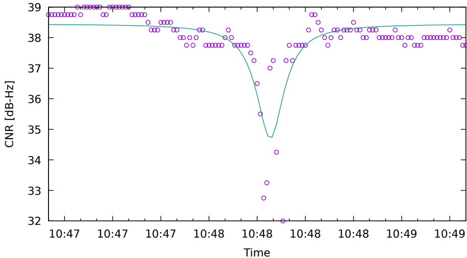
CNR fit for C21 on Xiaomi11T - drive 5 (DOY263)
