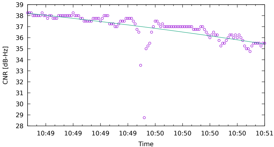
CNR fit for C21 on Xiaomi11T - drive 6 (DOY263)
