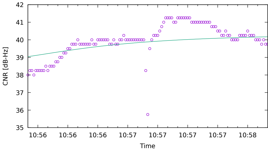
CNR fit for C33 on Xiaomi11T - drive 10 (DOY263)
