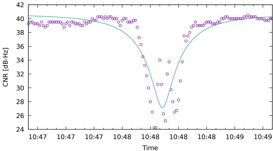
CNR fit for E04 on Xiaomi11T - drive 5 (DOY263)
