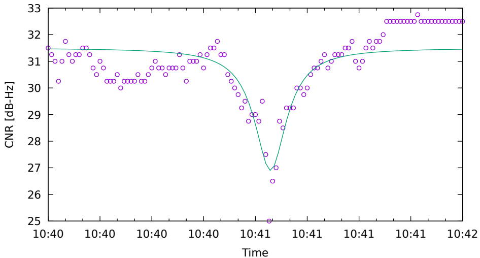
CNR fit for E19 on Xiaomi11T - drive 1 (DOY263)
