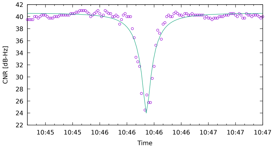
CNR fit for E33 on Xiaomi11T - drive 4 (DOY263)
