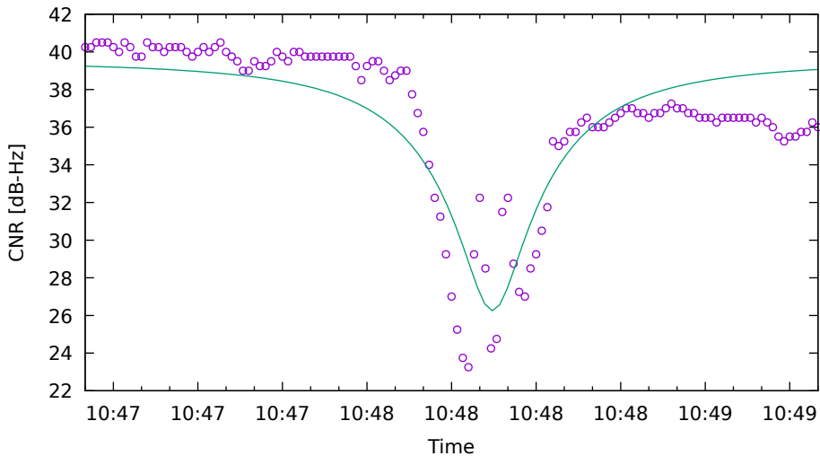
CNR fit for E33 on Xiaomi11T - drive 5 (DOY263)
