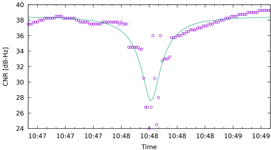
CNR fit for G19 on Xiaomi11T - drive 5 (DOY263)
