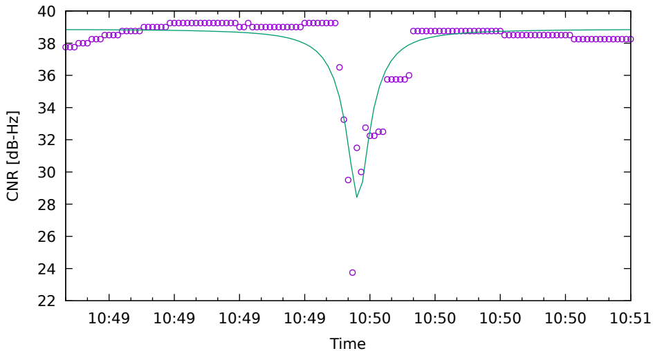
CNR fit for G19 on Xiaomi11T - drive 6 (DOY263)
