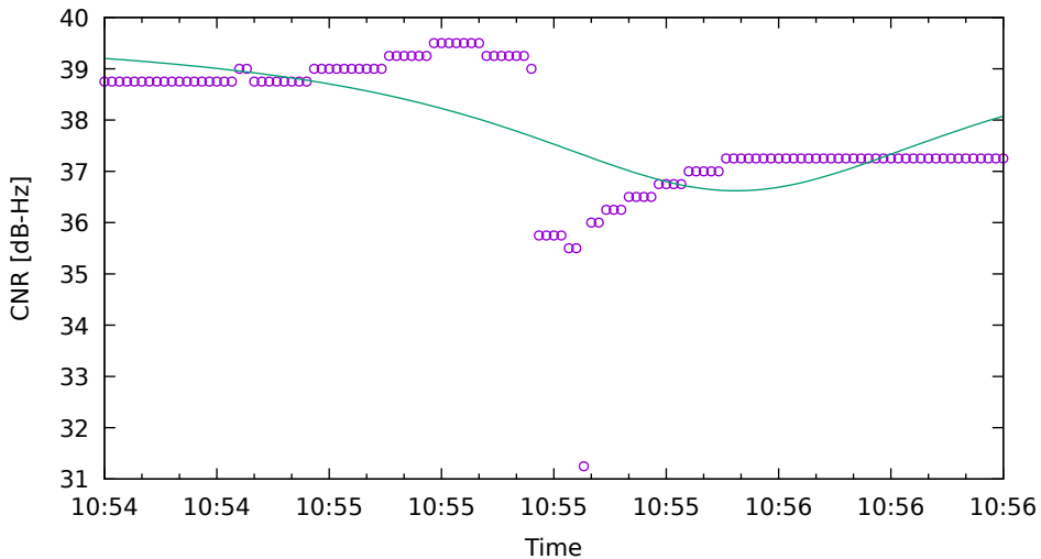
CNR fit for G19 on Xiaomi11T - drive 9 (DOY263)
