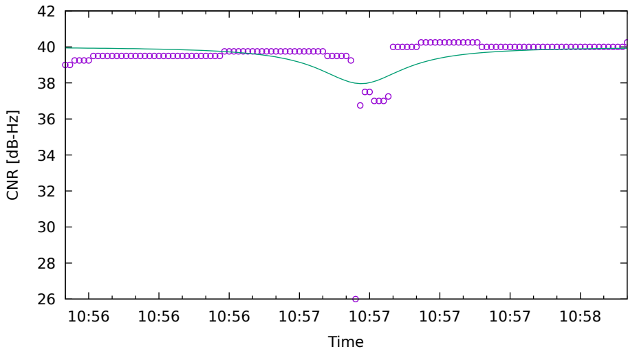
CNR fit for G21 on Xiaomi11T - drive 10 (DOY263)
