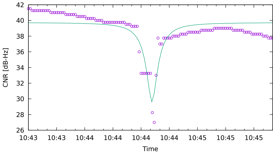
CNR fit for G21 on Xiaomi11T - drive 3 (DOY263)
