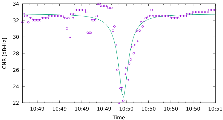
CNR fit for G22 on Xiaomi11T - drive 6 (DOY263)
