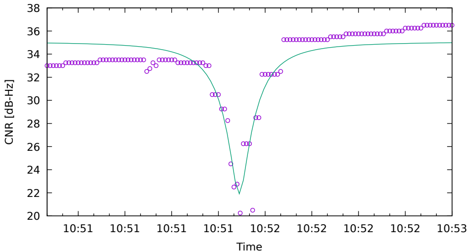
CNR fit for G22 on Xiaomi11T - drive 7 (DOY263)
