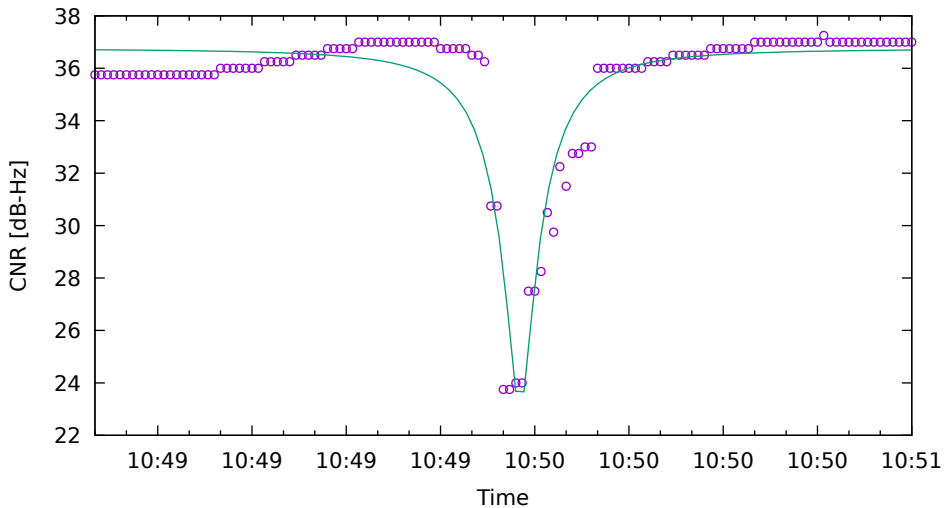
CNR fit for G31 on Xiaomi11T - drive 6 (DOY263)
