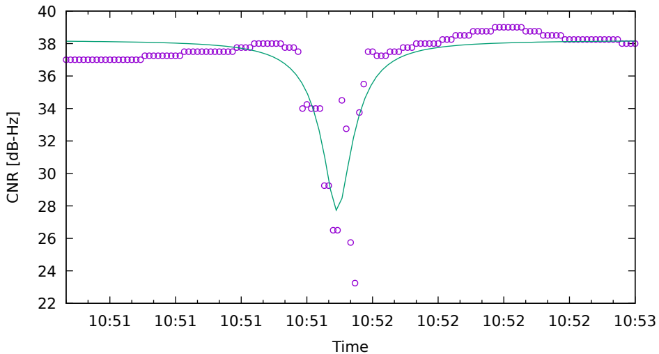
CNR fit for G31 on Xiaomi11T - drive 7 (DOY263)
